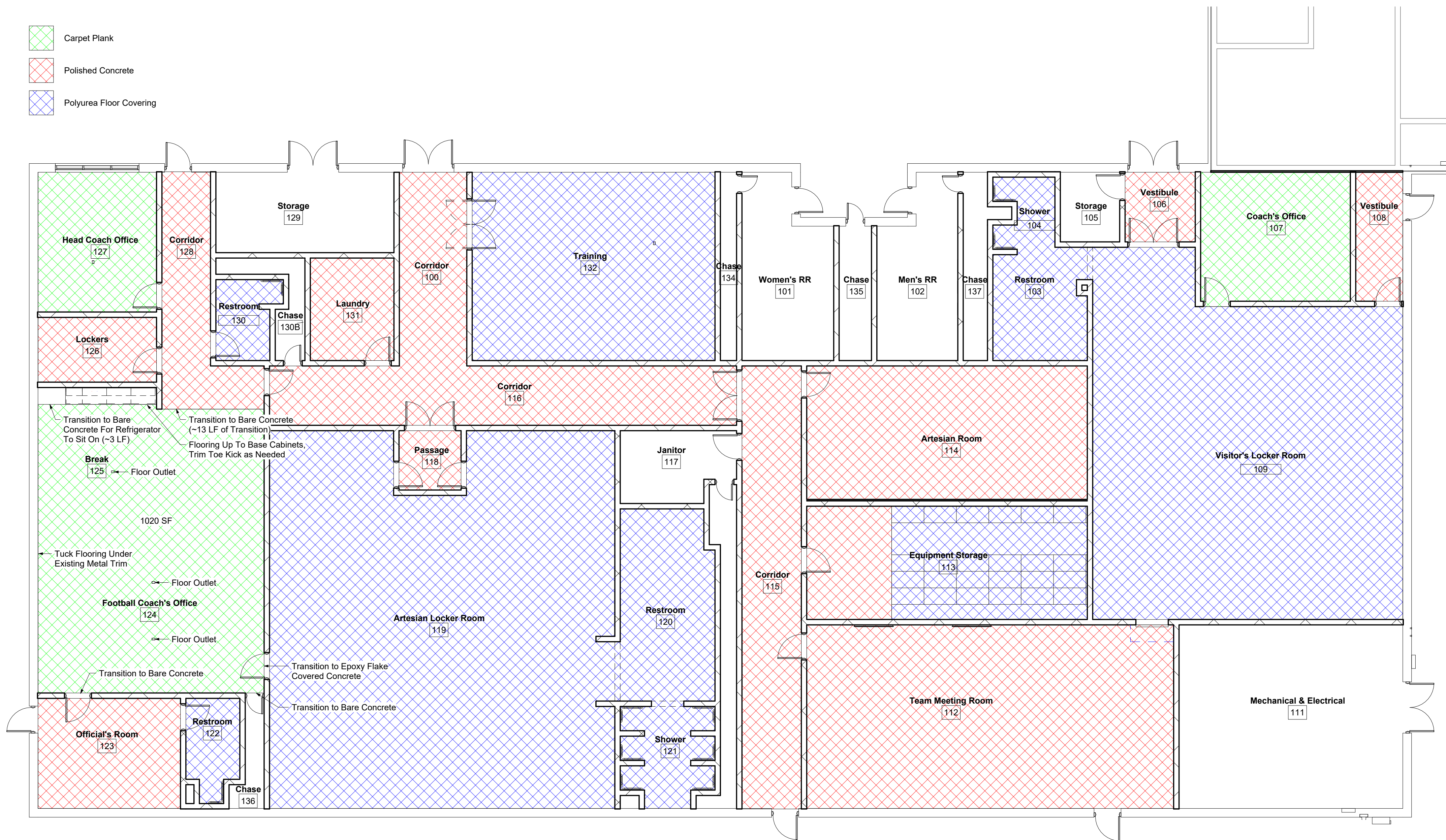
1 Floor Covering - Plan 1/8" = 1'-0"
